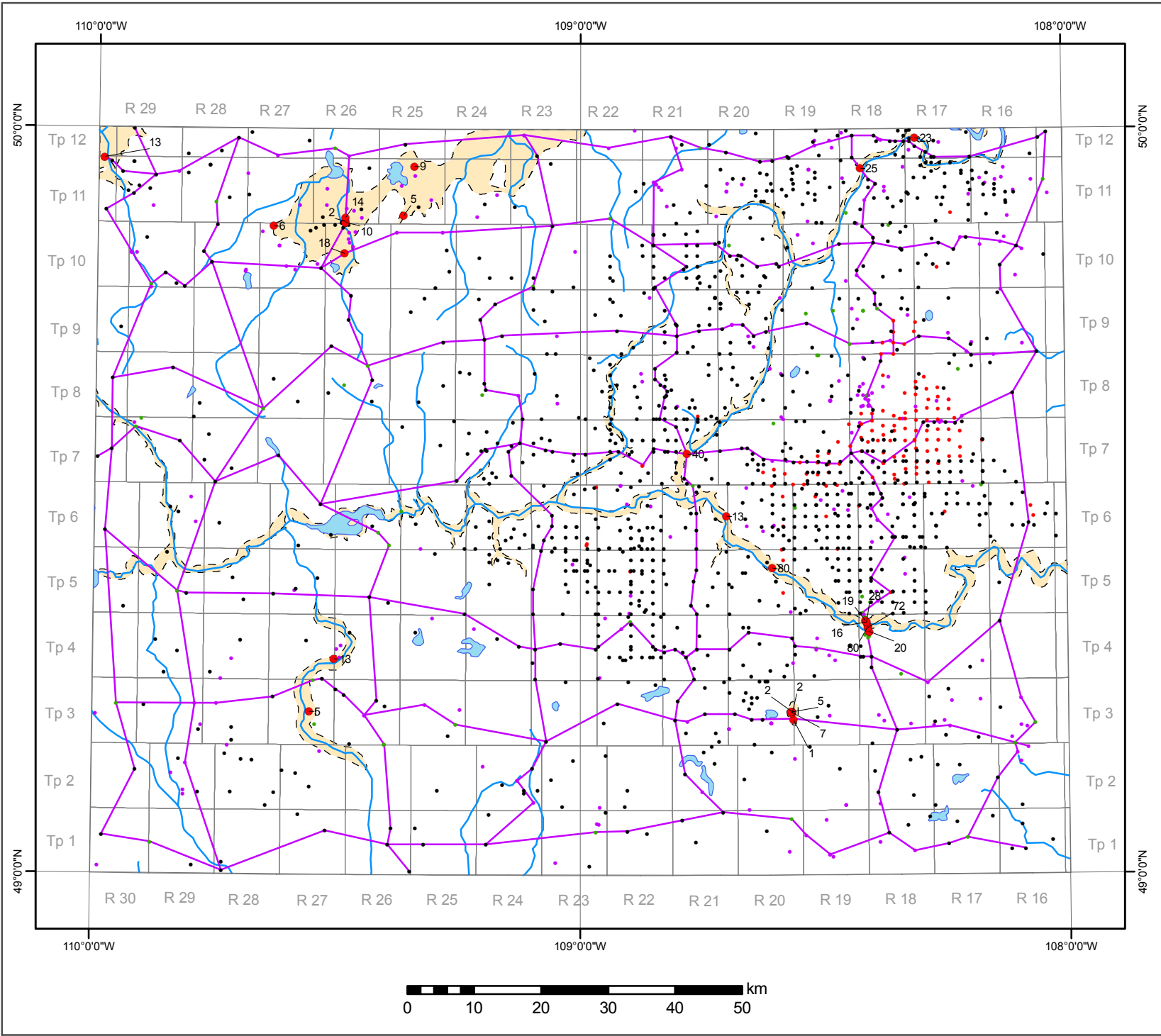
Extent and thickness of surficial aquifers in the Cypress Lake area
