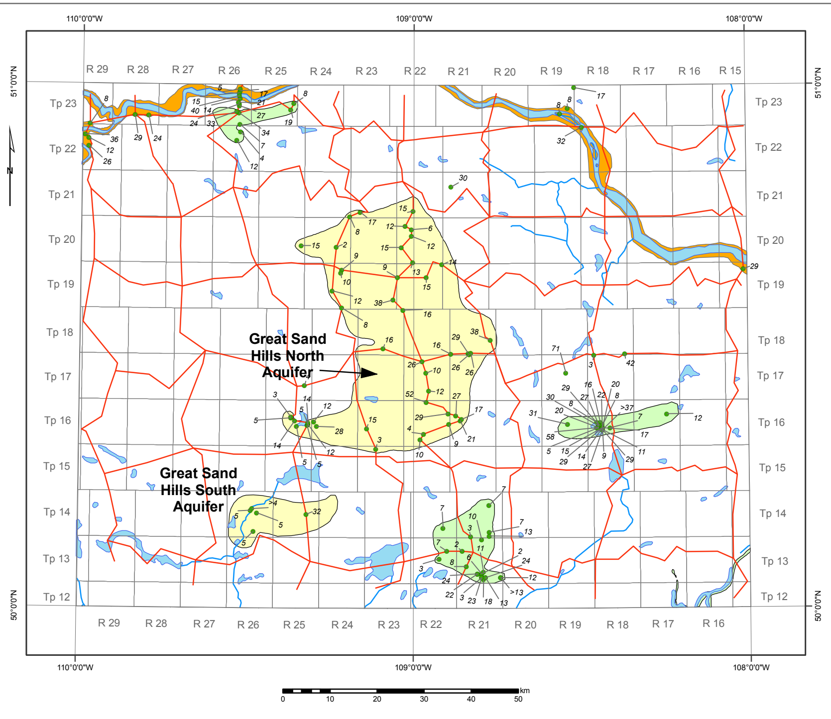
Extent and thickness of surficial aquifers in the Prelate area
