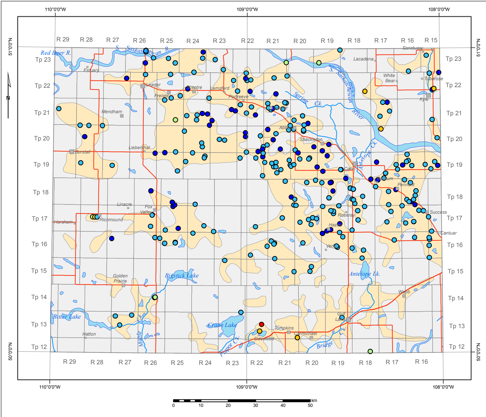
Aquifer vulnerability index (AVI) of the Saskatoon Group aquifers in the Prelate area
