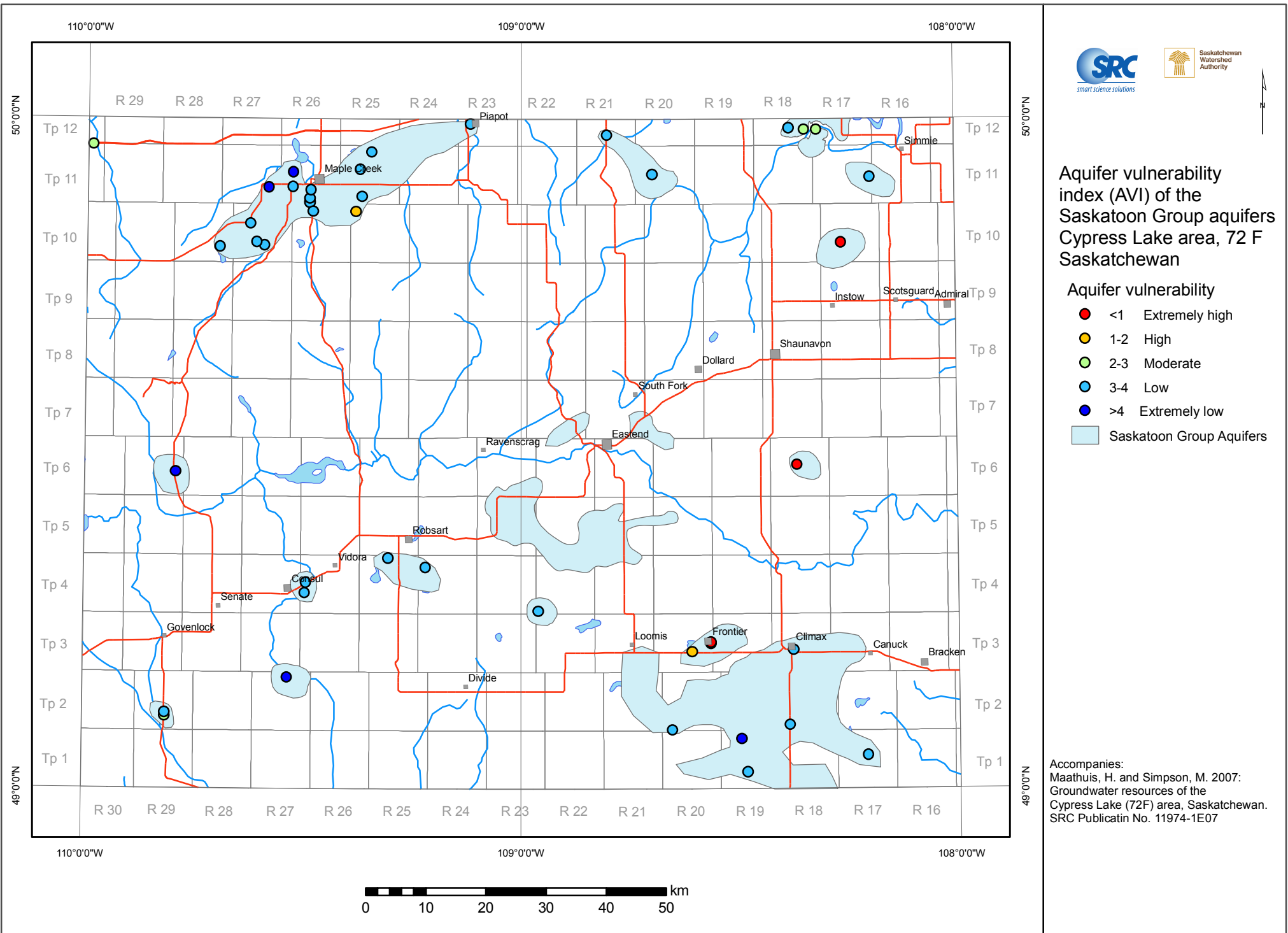
Aquifer vulnerability index of the Saskatoon Group aquifers in the Cypress Lake area
