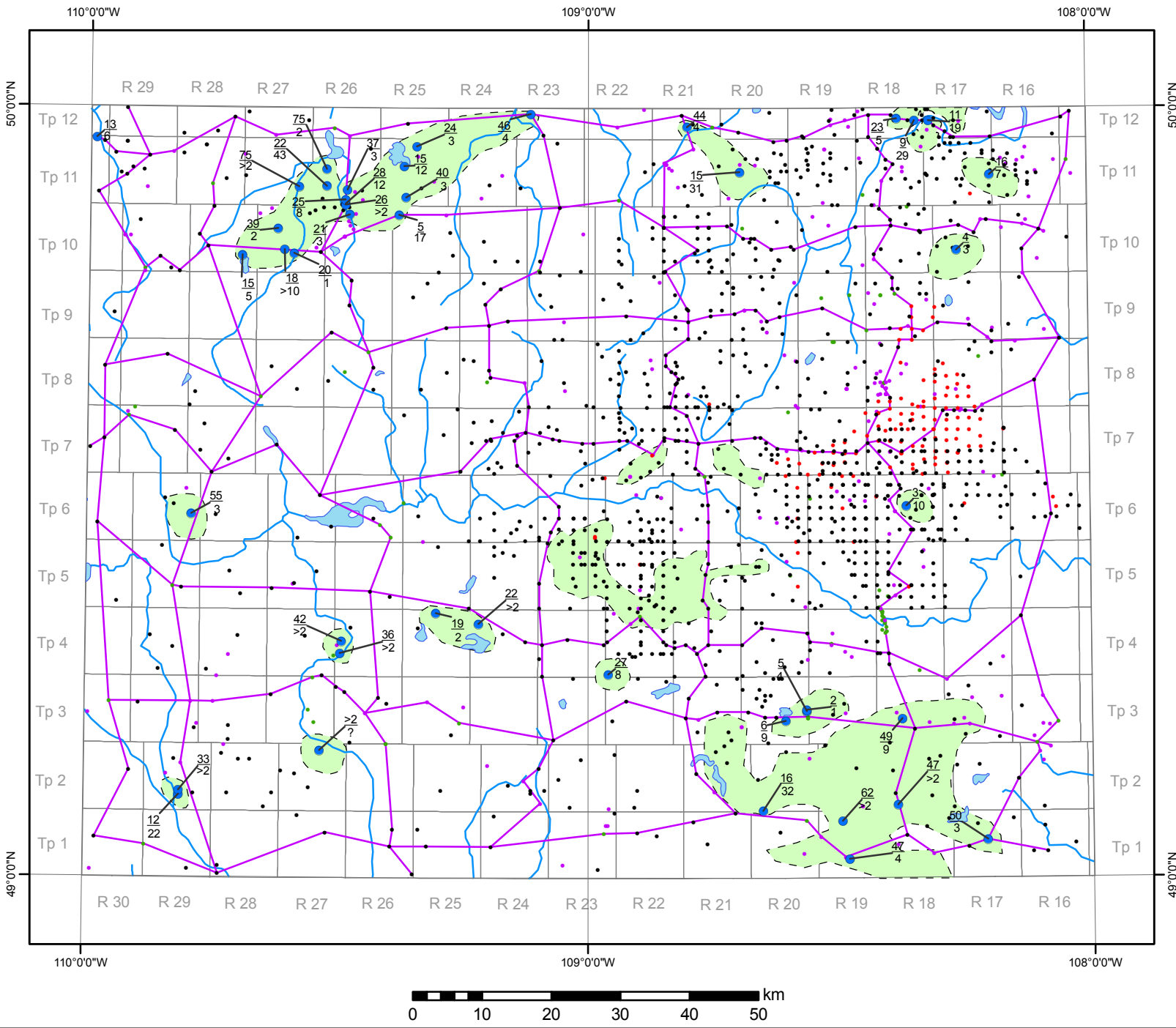
Extent, depth to and thickness of the Saskatoon Group aquifers in the Cypress Lake area
