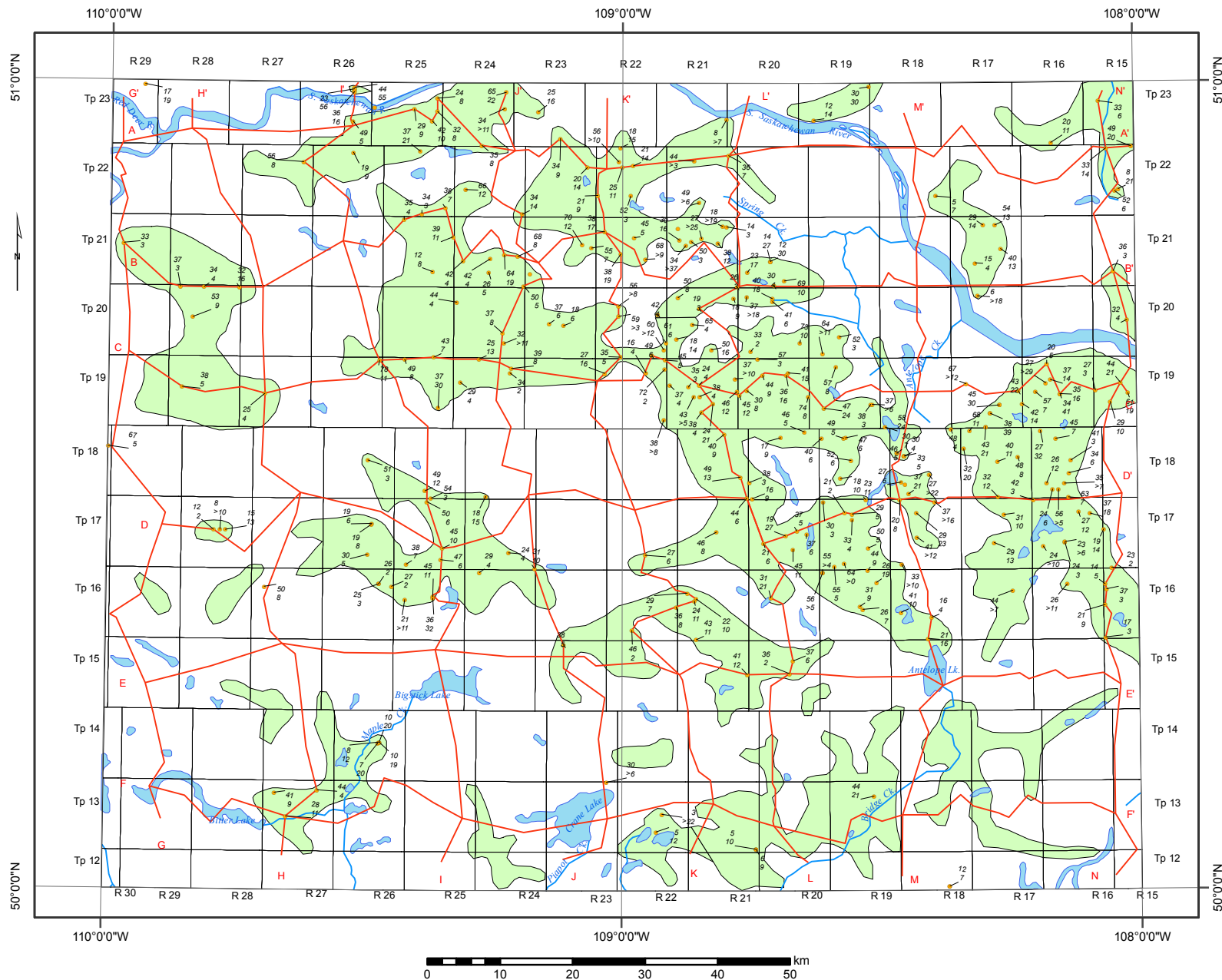
Extent, depth to and thickness of the Saskatoon Group aquifers
