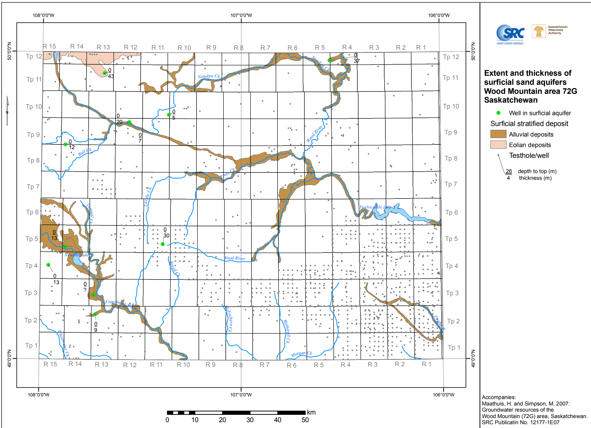
Extent and thickness of surficial deposits in the Wood Mountain area
