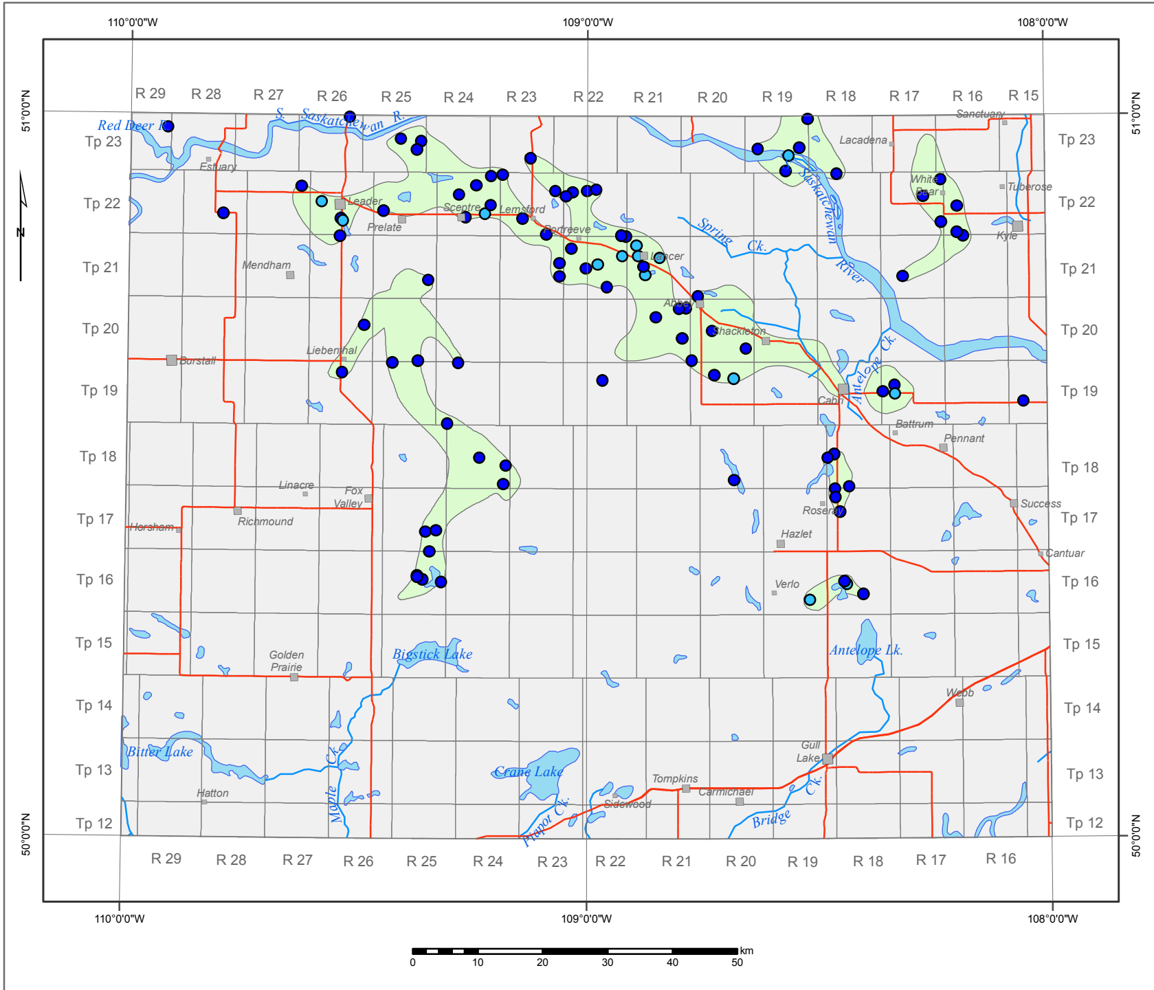
Aquifer vulnerability index (AVI) of the Sutherland Group aquifers in the Prelate area
