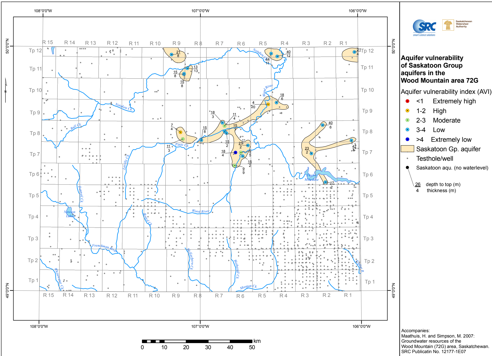
Aquifer vulnerability index (AVI) of the Saskatoon Group aquifers in the Wood Mountain area
