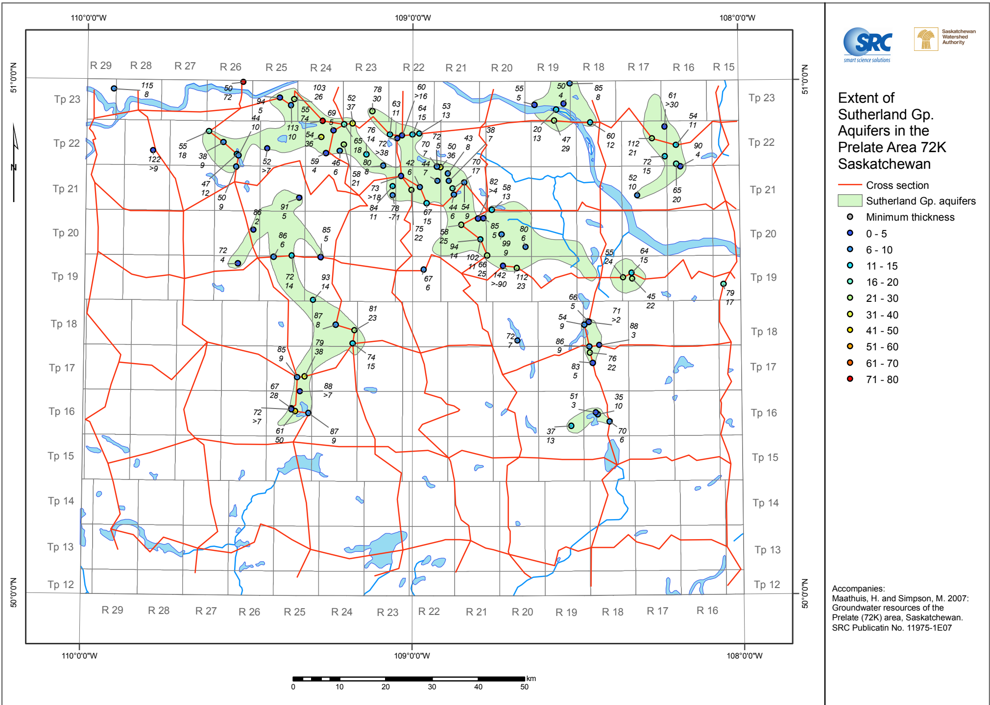
Extent, depth to and thickness of the Sutherland Group aquifers in the Prelate area
