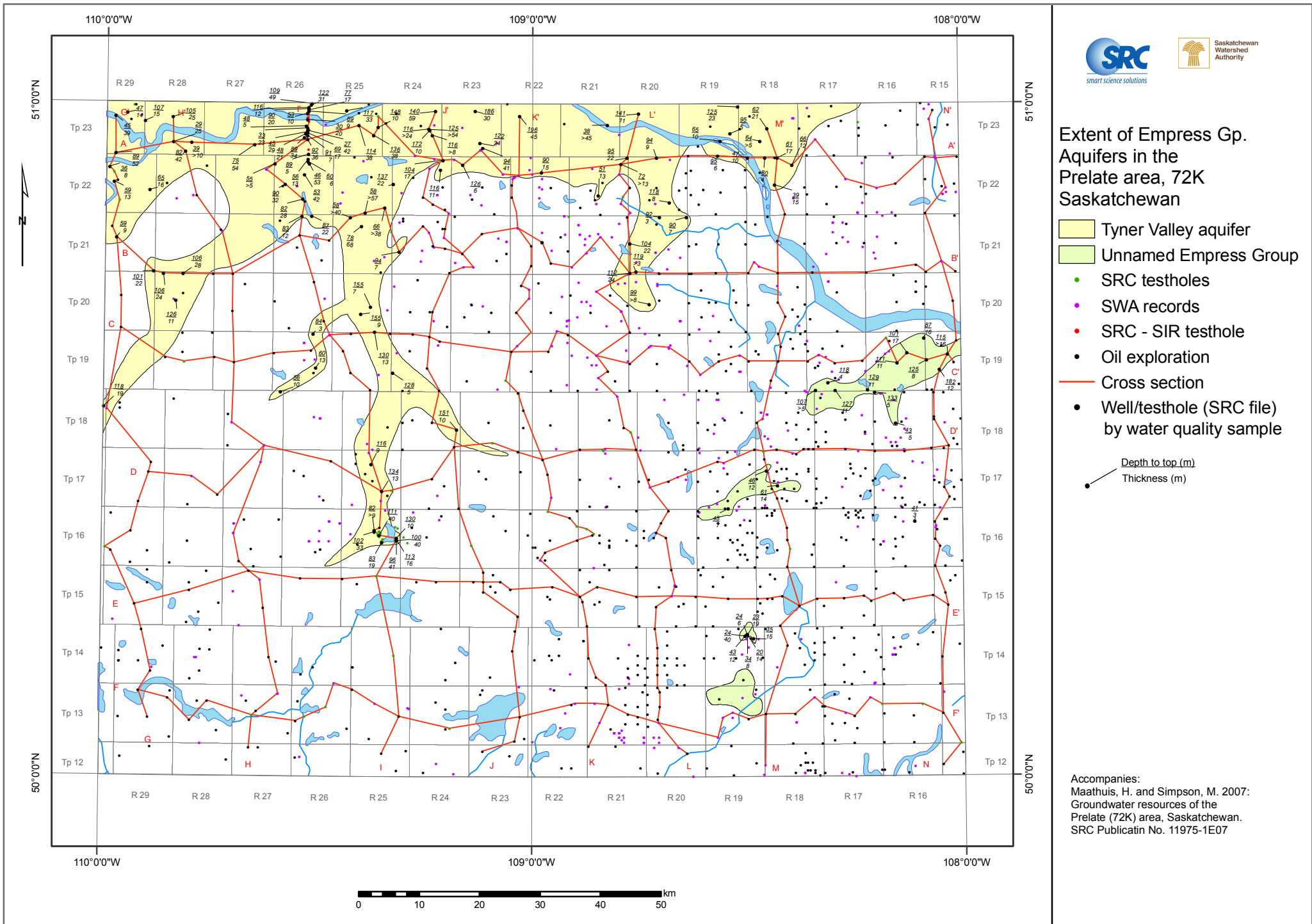
Extent, depth to and thickness of aquifers formed by Empress Group sediments in the Prelate area
