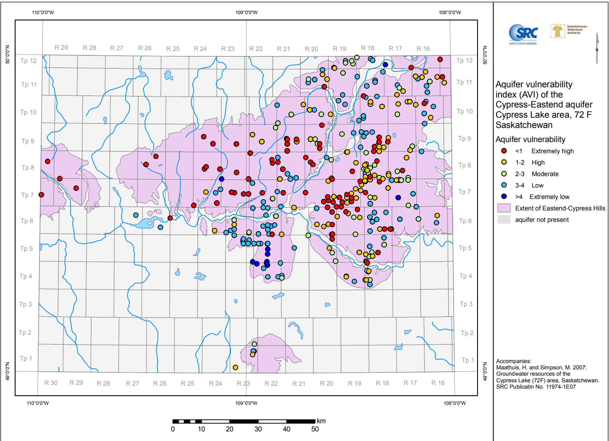
Aquifer vulnerability index for the Eastend to Cypress Hills aquifer in the Cypress Lake area
