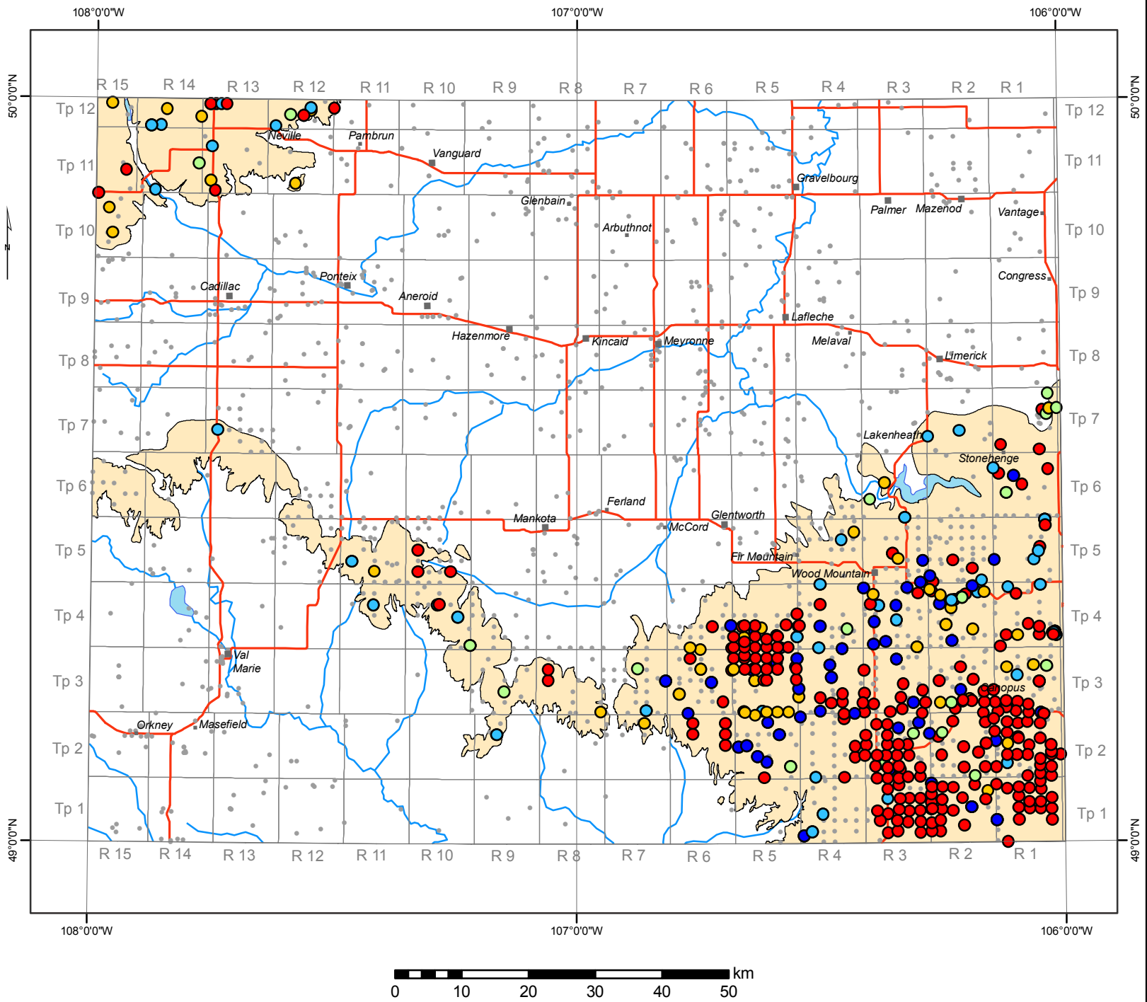
Aquifer vulnerability index (AVI) of the Eastend-Wood Mountain aquifer in the Wood Mountain area
