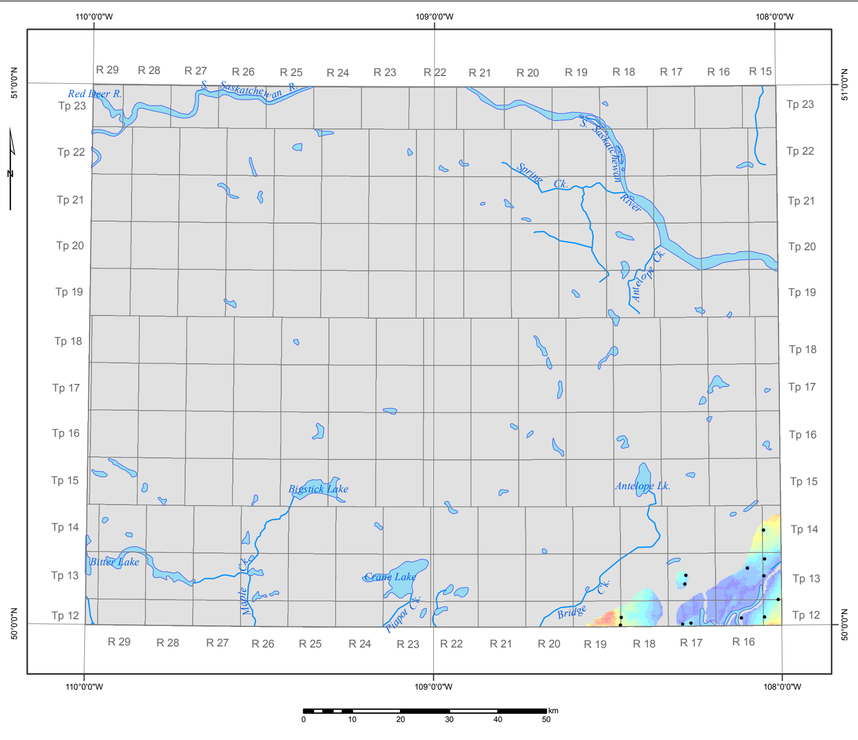
Thickness of the Eastend-Cypress Hills aquifer in the Prelate area
