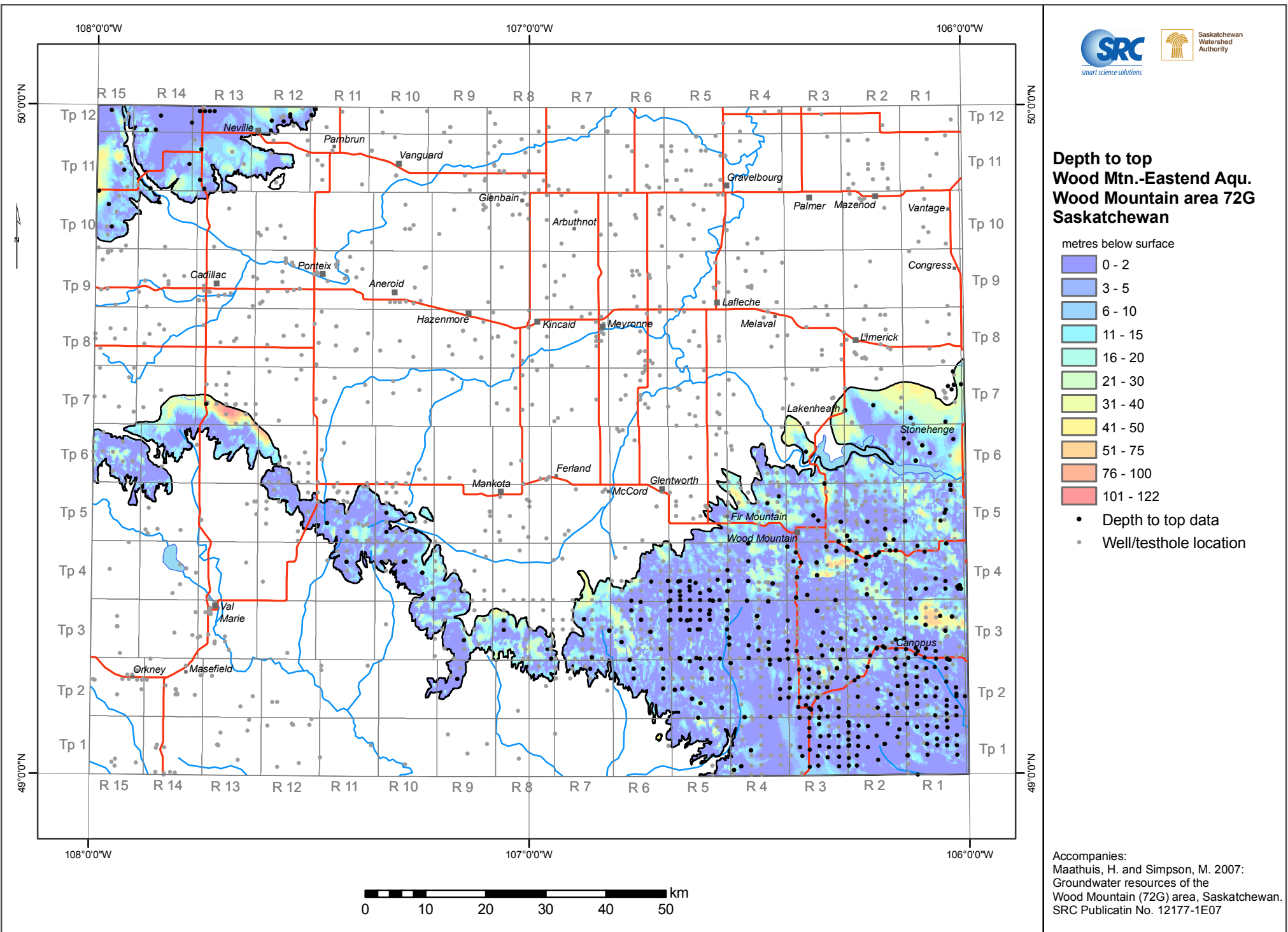
Extent and depth to the Eastend-Wood Mountain aquifer in the Wood Mountain area
