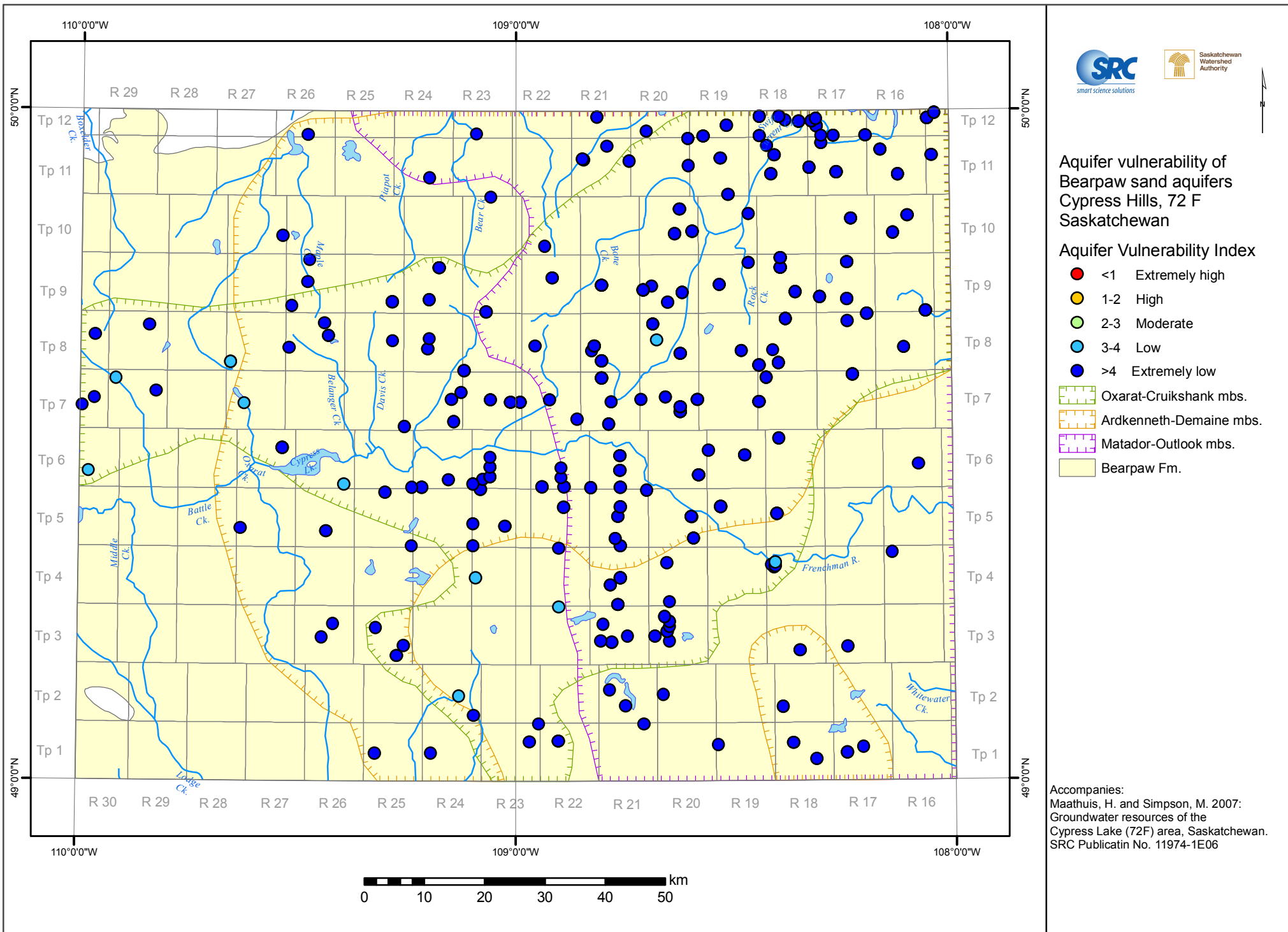
Aquifer vulnerability index for the Bearpaw sand members aquifer in the Cypress Lake area
