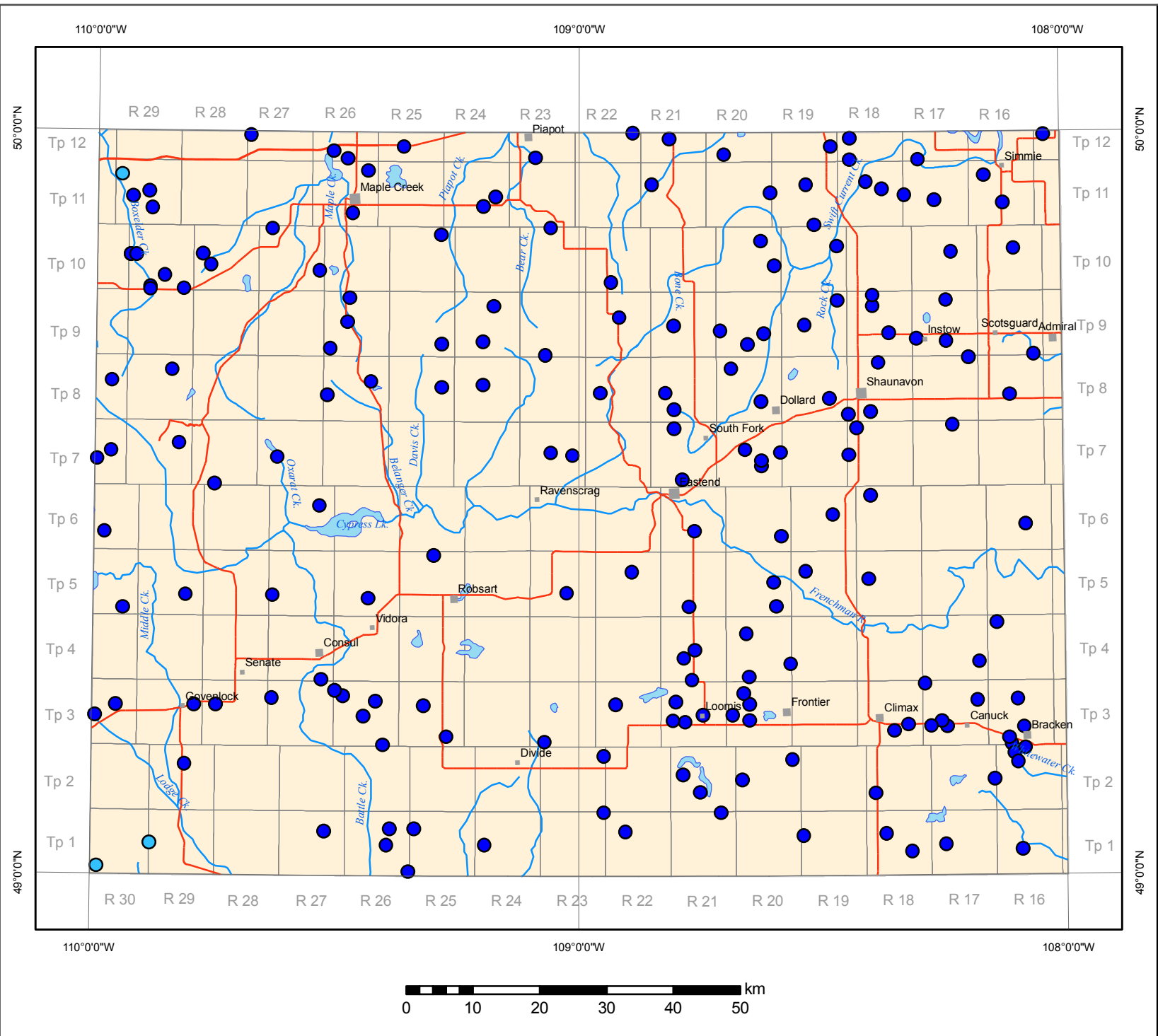
Aquifer vulnerability index for the Judith River aquifer in the Cypress Lake area
