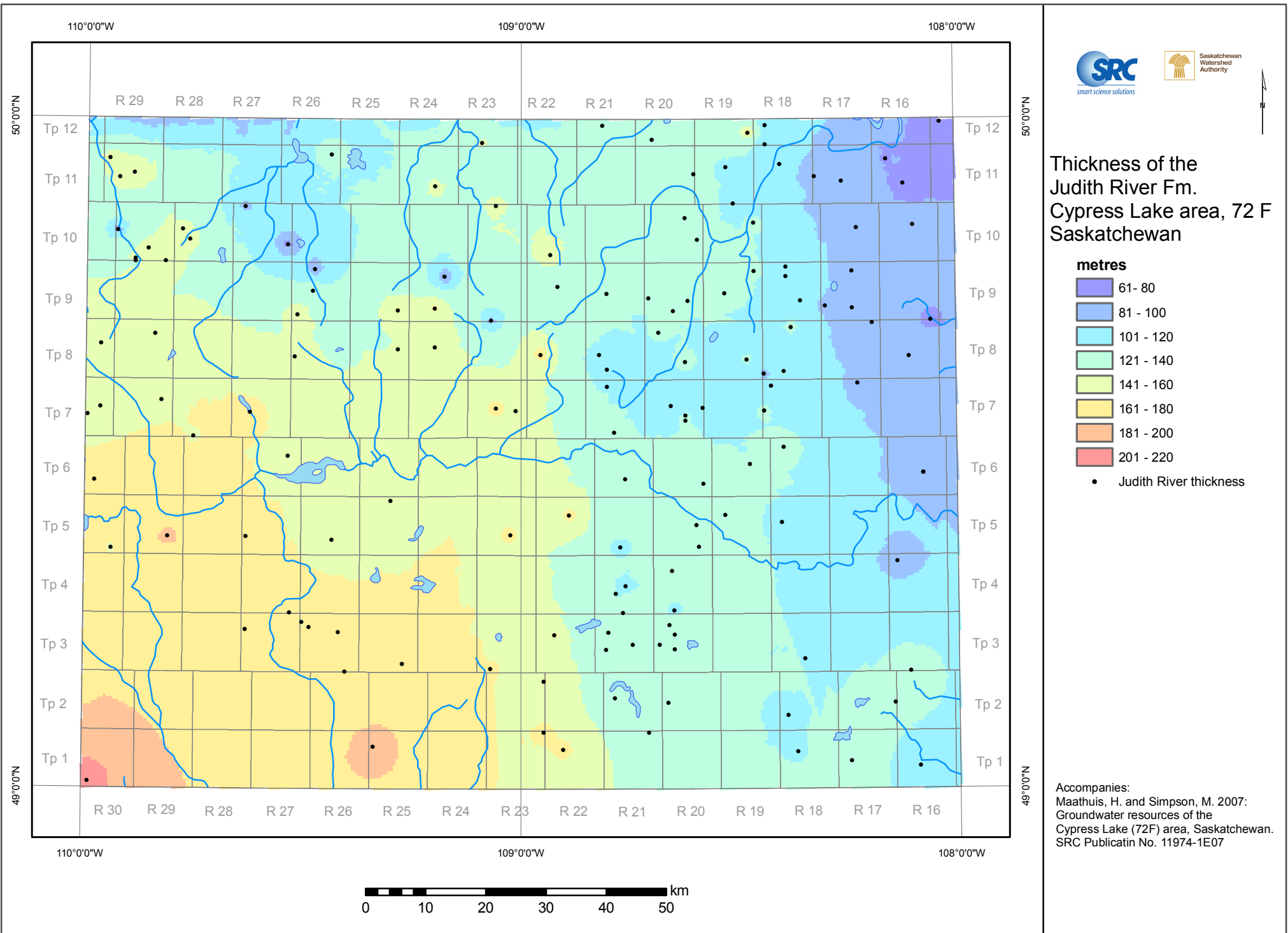
Thickness of the Judith River Formation in the Cypress Lake area
