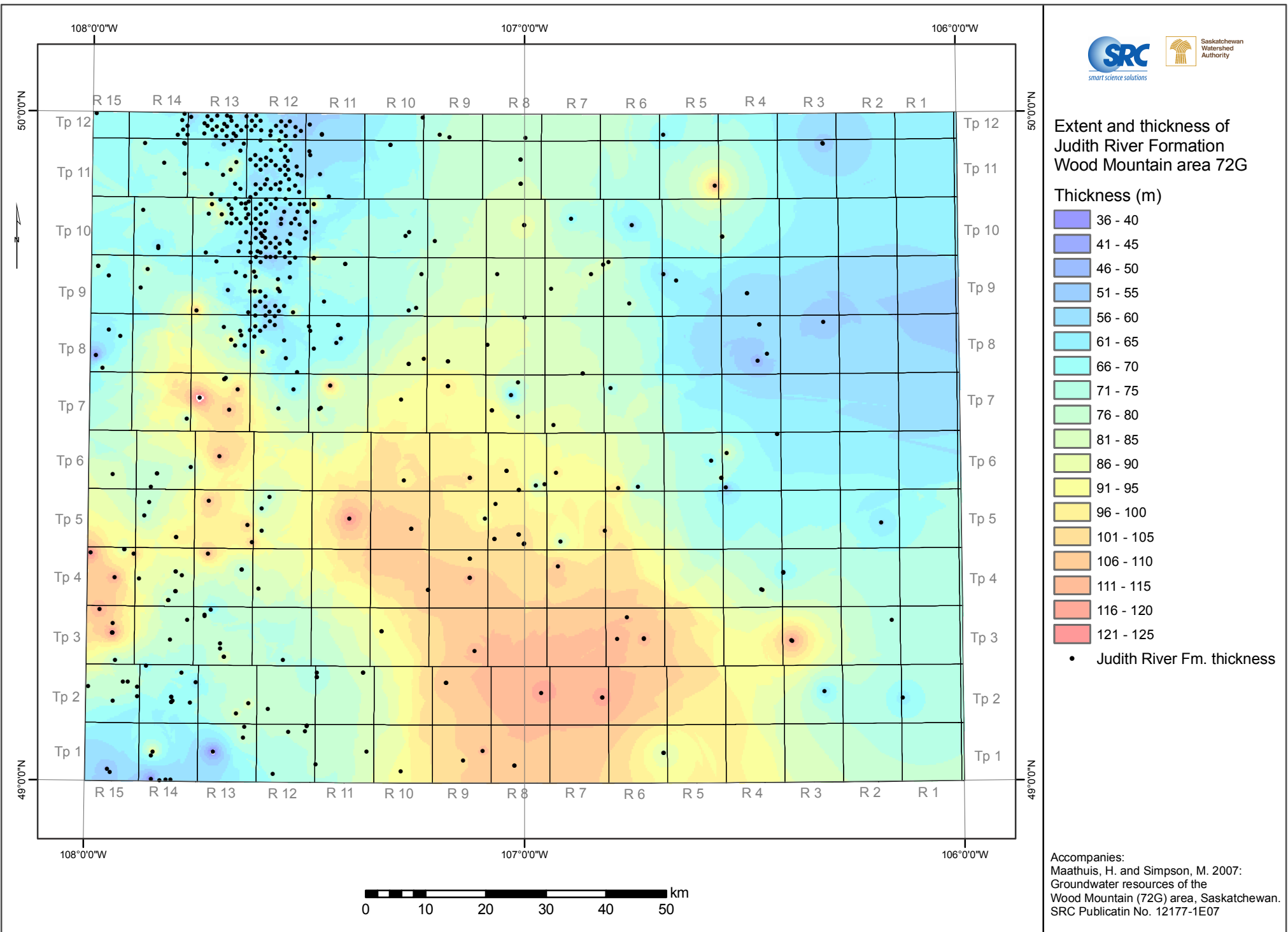
Thickness of the Judith River Formation in the Wood Mountain area
