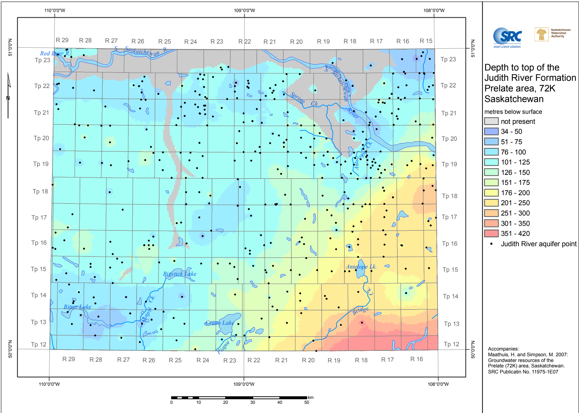
Extent and depth to the top of the Judith River Formation in the Prelate area
