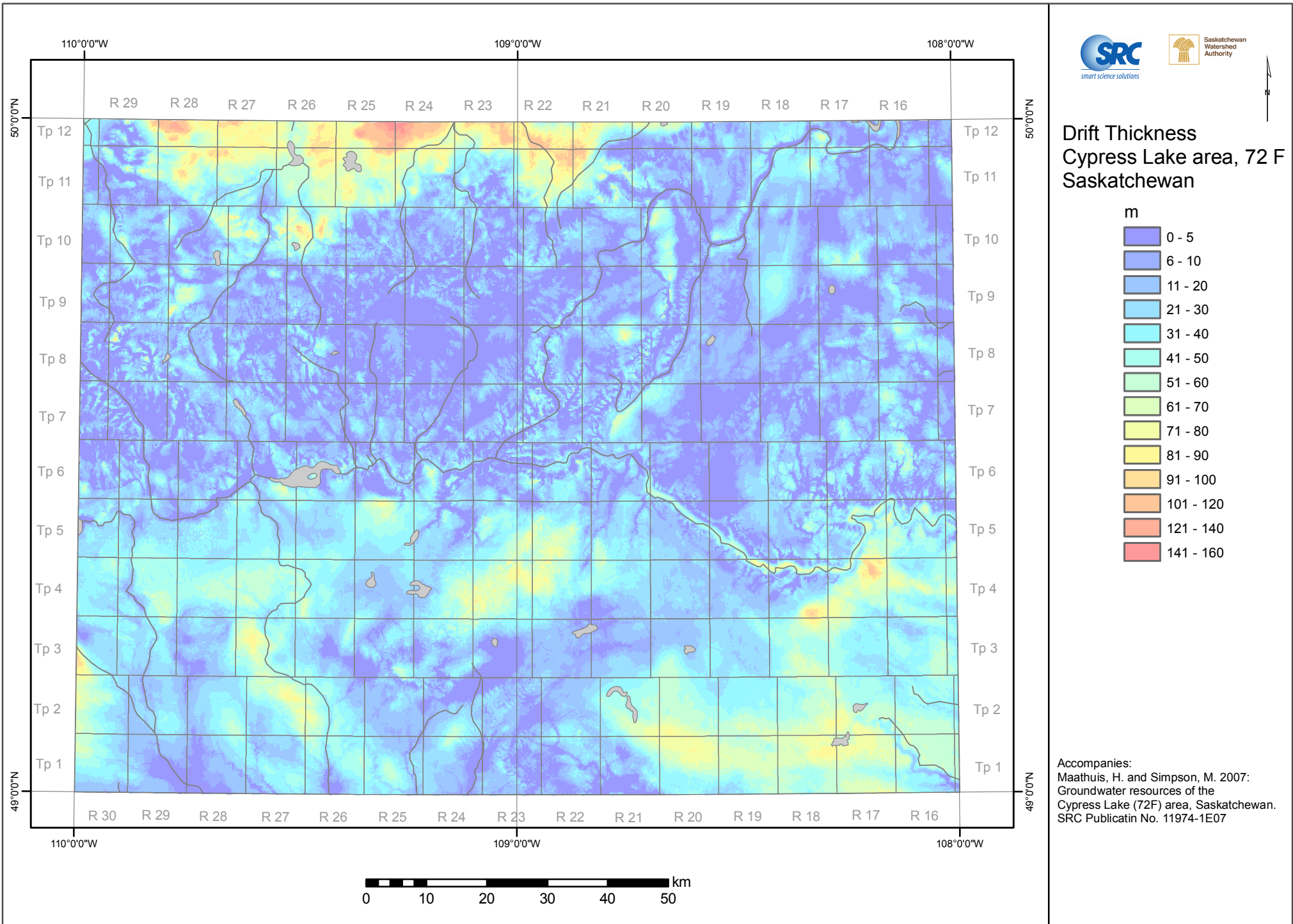
Thickness of the drift in the Cypress Lake area
