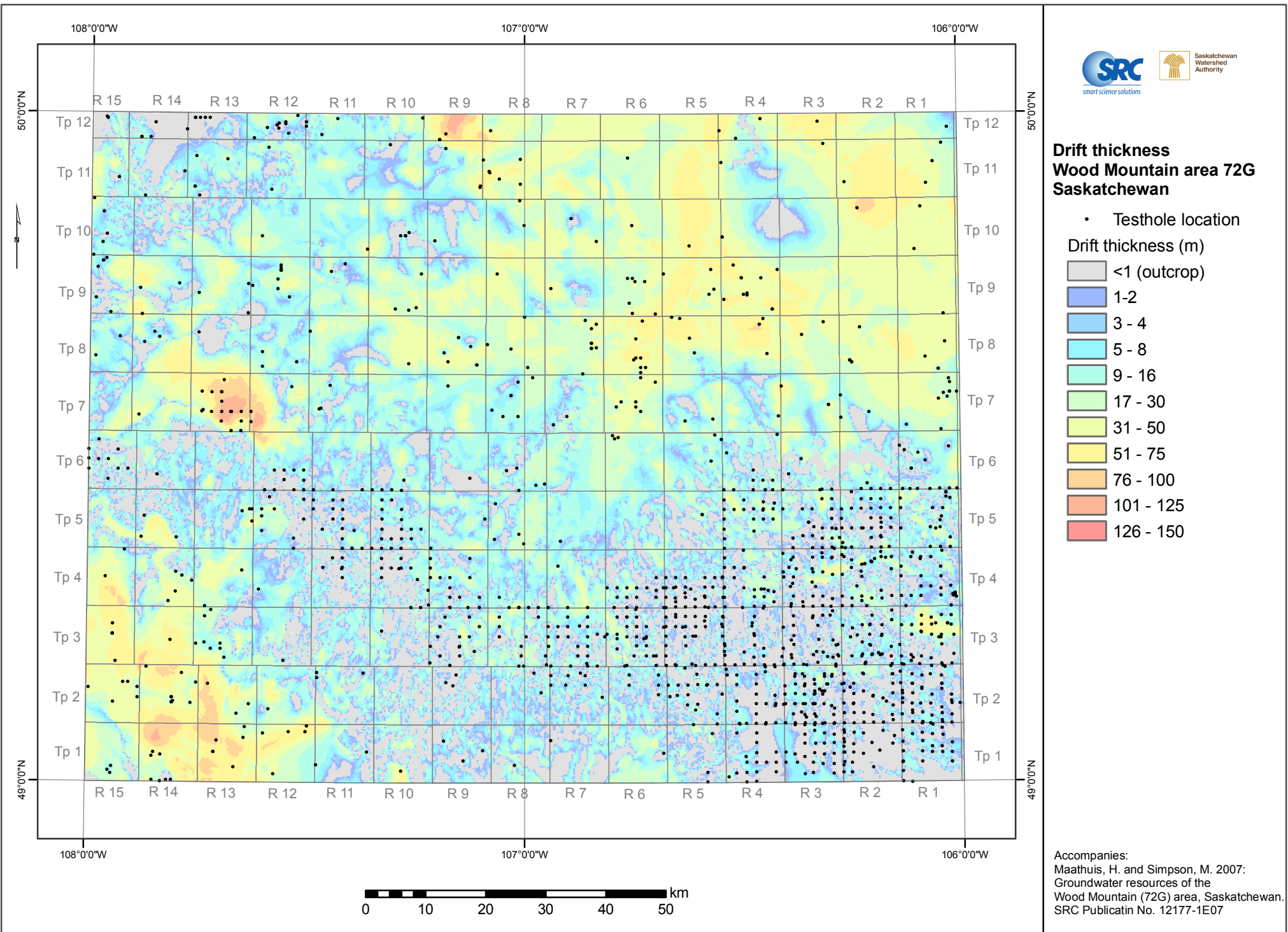
Thickness of the drift in the Wood Mountain area
