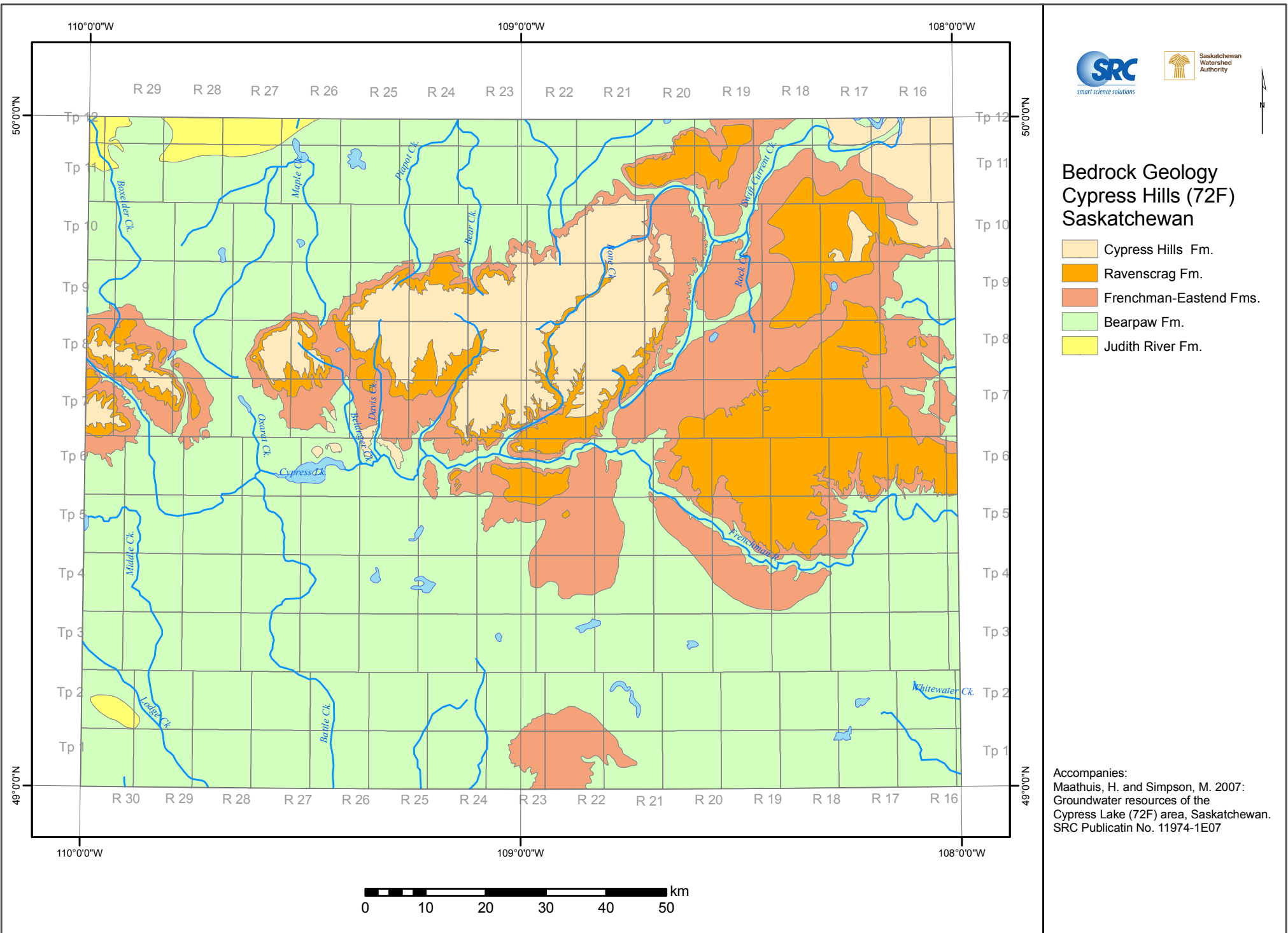
Bedrock geology of the Cypress Lake area
