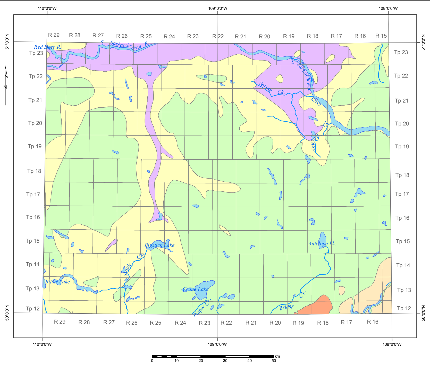
Bedrock geology of the Prelate area
