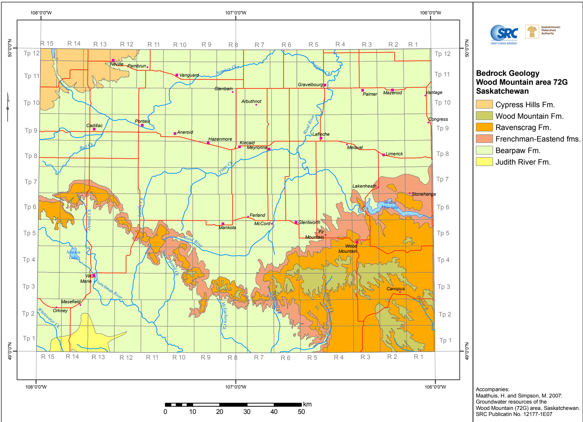
Bedrock geology of the Wood Mountain area
