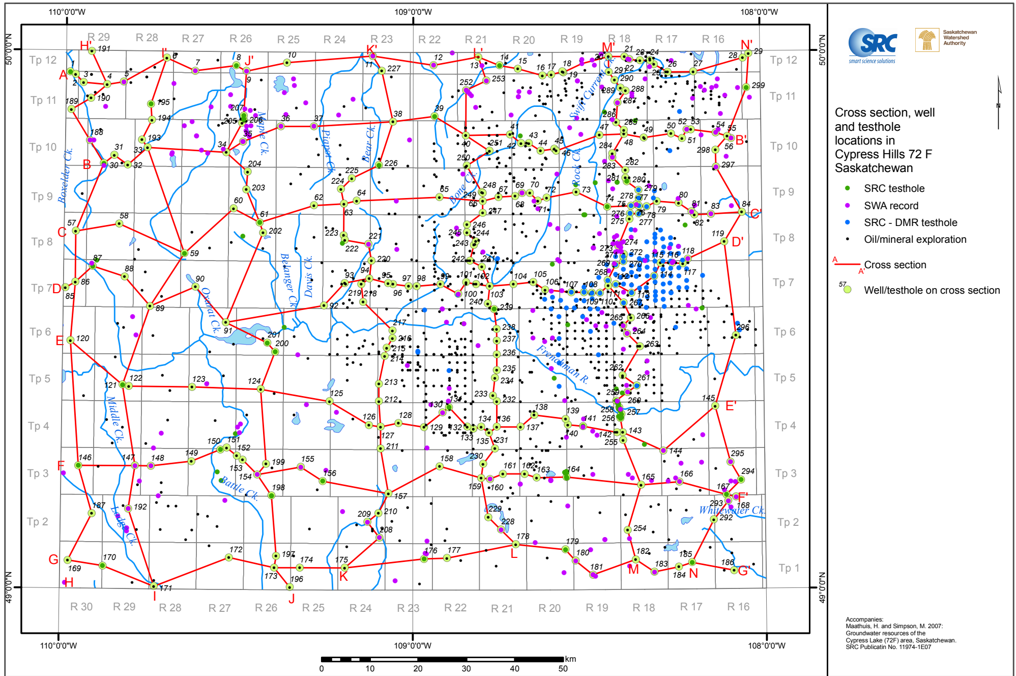
Locations of testholes and cross section lines in teh Cypress Lake map sheet area
