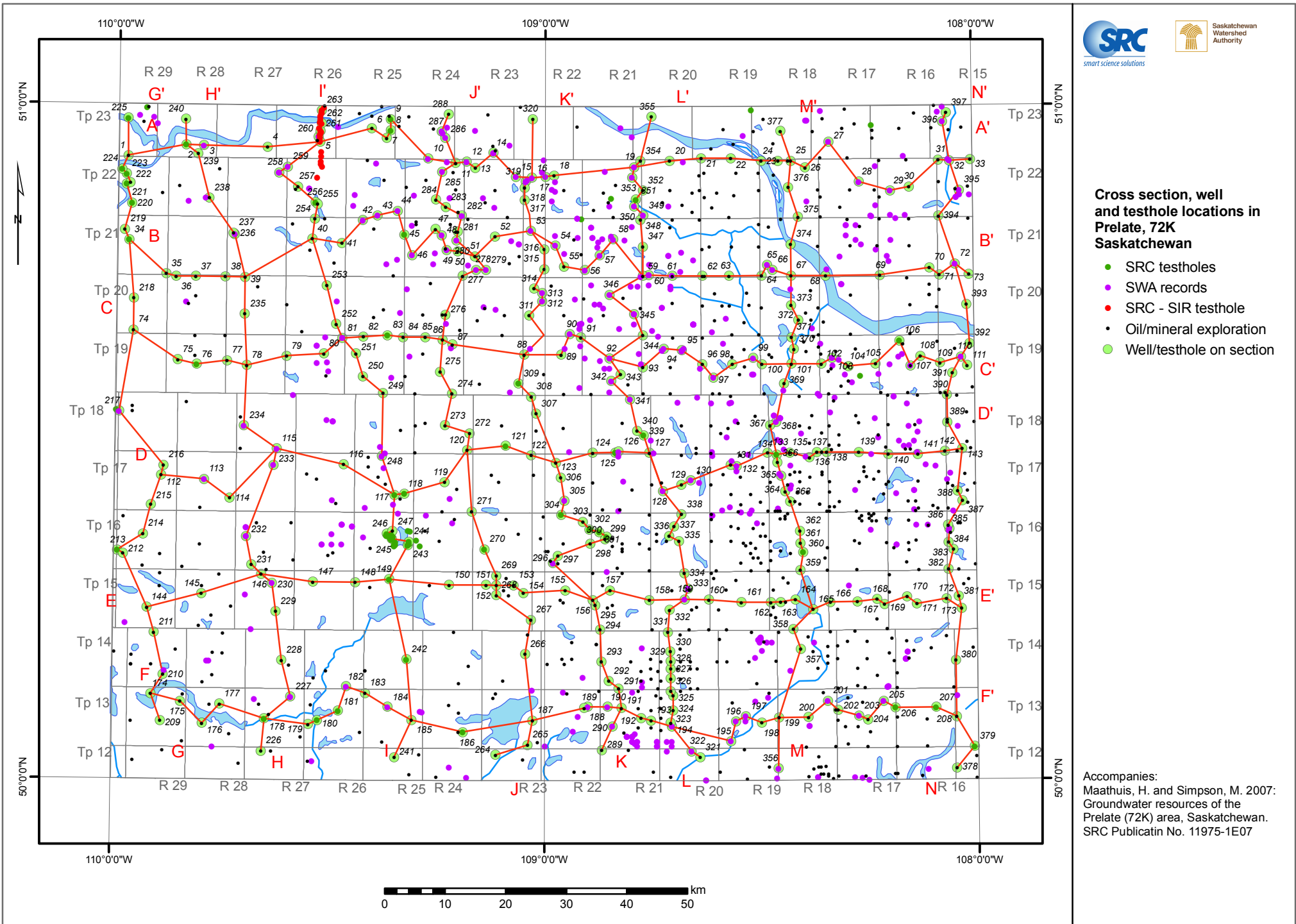
Locations of testholes and cross sections lines in the Prelate map sheet area
