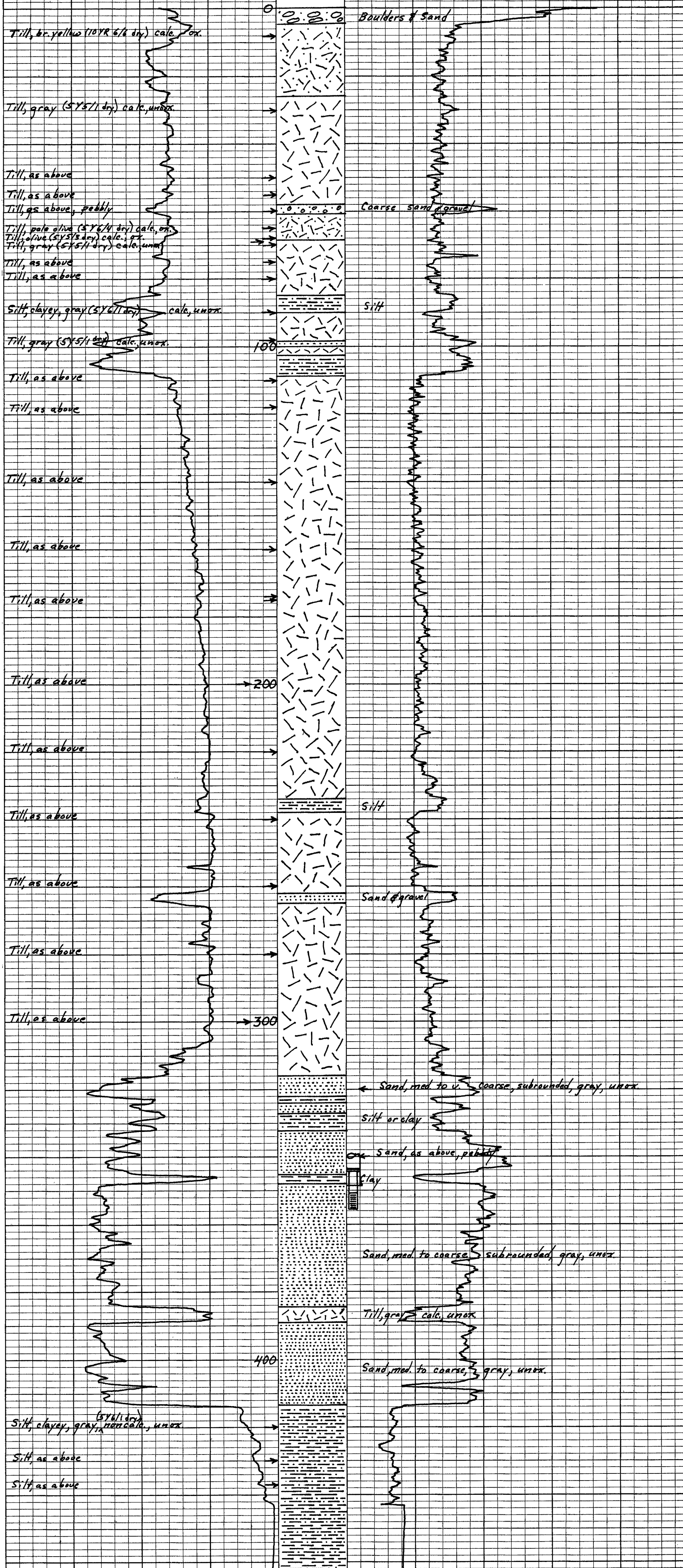
E-log, sidehole Core Descriptions & Driller's Log From WARMAN Testhole 1965 NE-13-9-39-5-W-3 Elevation 1700' Drillers: Maik & Soloninko Geologist: E.A. Christiansen
