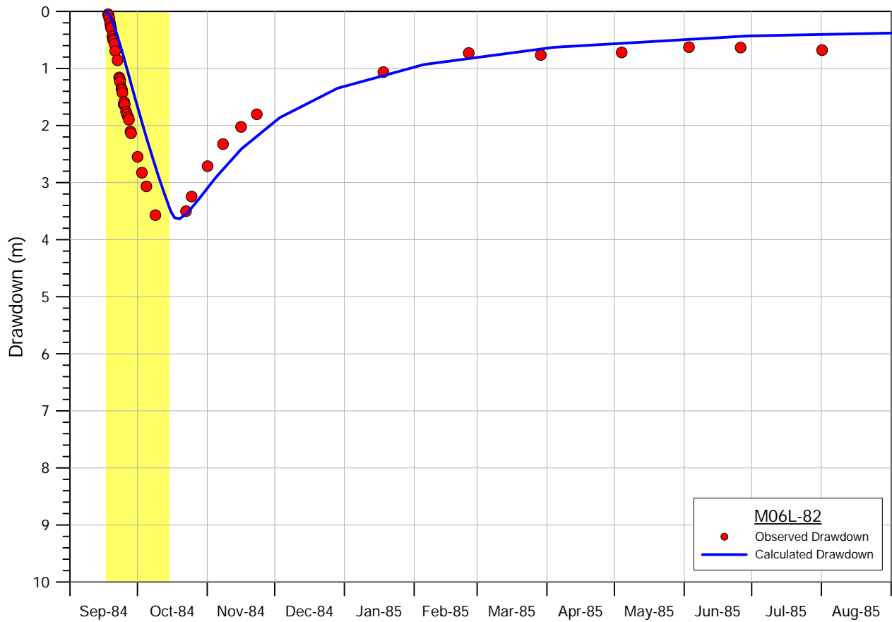
Figure D.4: Drawdown in wells M17U-84 and M06L-82 during 1984 pumping test
