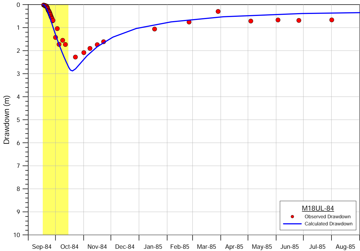
Figure D.6: Drawdown in wells M20U-84 and M18UL-84 during 1984 pumping test
