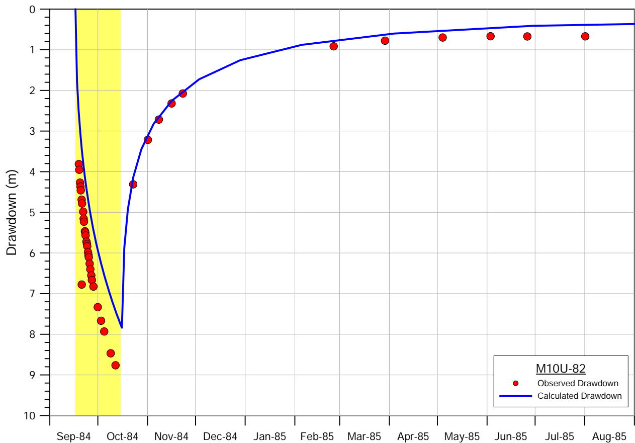
Figure D.2: Drawdown in wells M09L-82 and M10U-82 during 1984 pumping test
