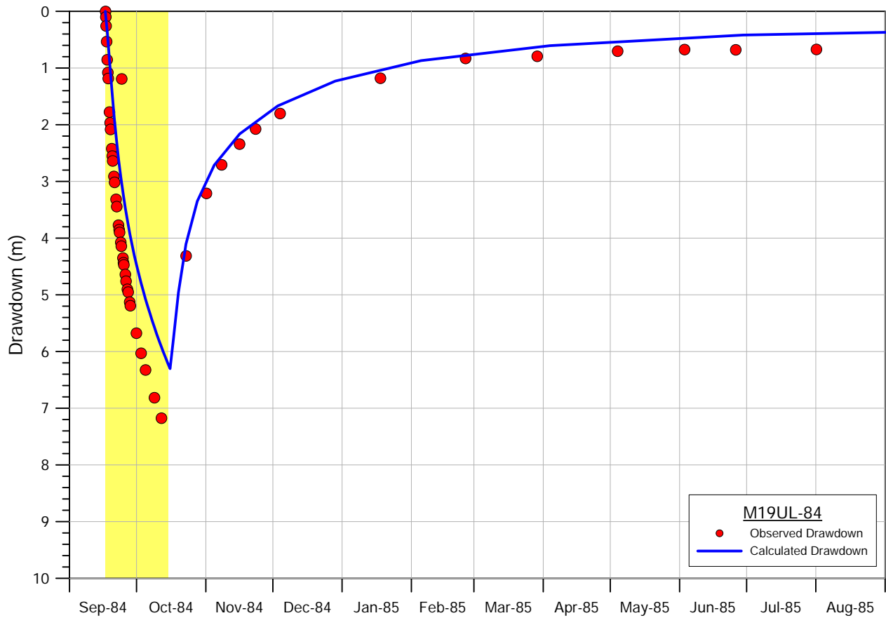
Figure D.1: Drawdown in wells M04U-82 and M19UL-84 during 1984 pumping test
