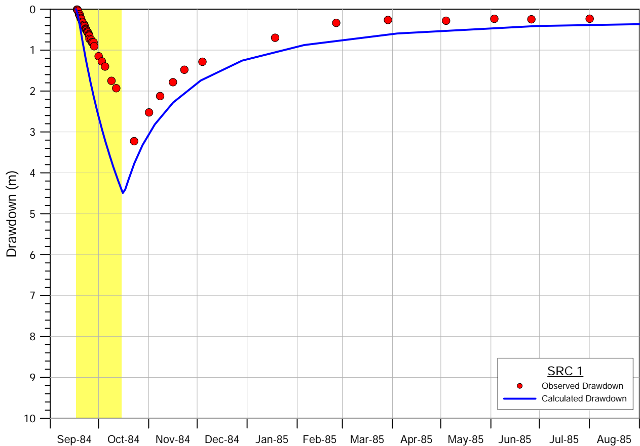
Figure D.5: Drawdown in wells M11L-84 and SRC 1 during 1984 pumping test
